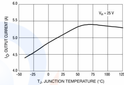
Figure 5. Current Limit
