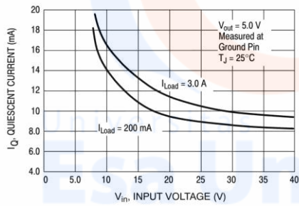
Figure 6. Quiescent Current
