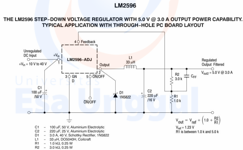
Figure 31. Schematic Diagram of the 5.0 V @ 3.0 A Step-Down Converter Using the LM2596-ADJ
