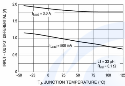
Figure 4. Dropout Voltage
