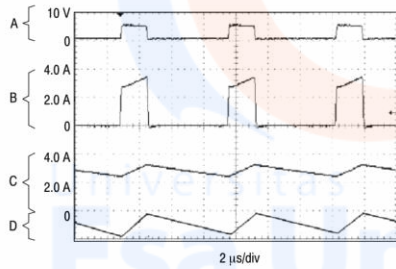
Figure 13. Switching Waveforms
